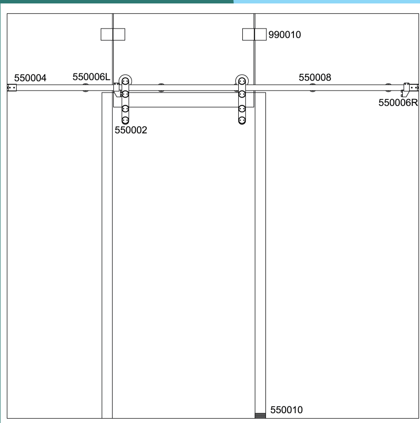
550002 Rollers
